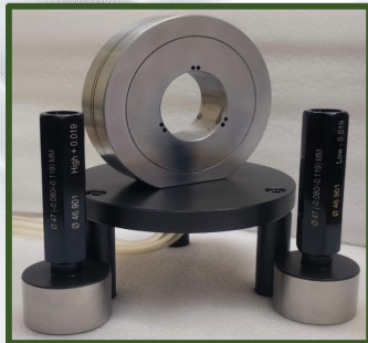
Special Air ring Gauges
